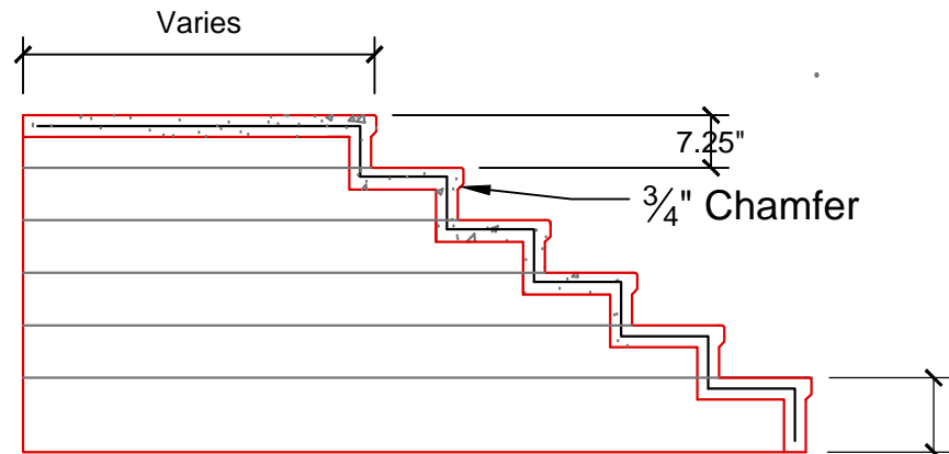
SECTION NOT TO SCALE
